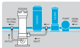
Illustration of Model 300 Feeder
