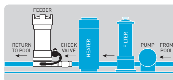
Illustration of Model 320 Feeder
