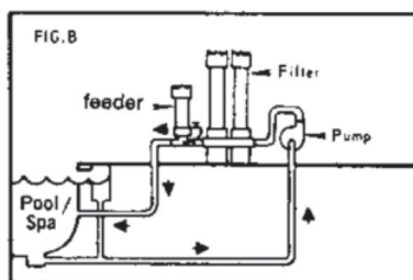
Typical Installation #320 without heater
