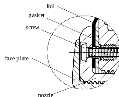
detail X
