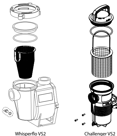
Strainer Pot Assembly
