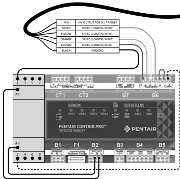
Figure 6: ControlPro Wiring Diagram
