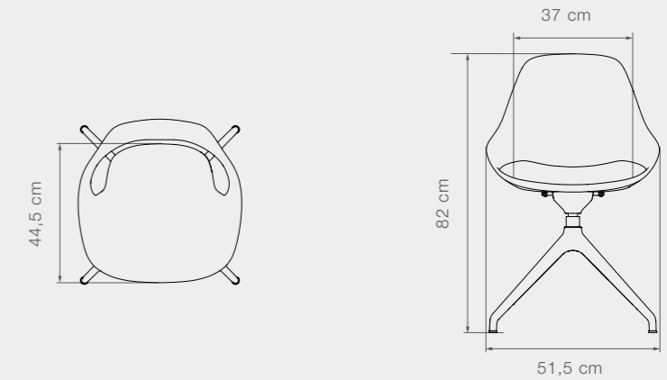
12902+12904 FALK Chair with four star return swivel base
