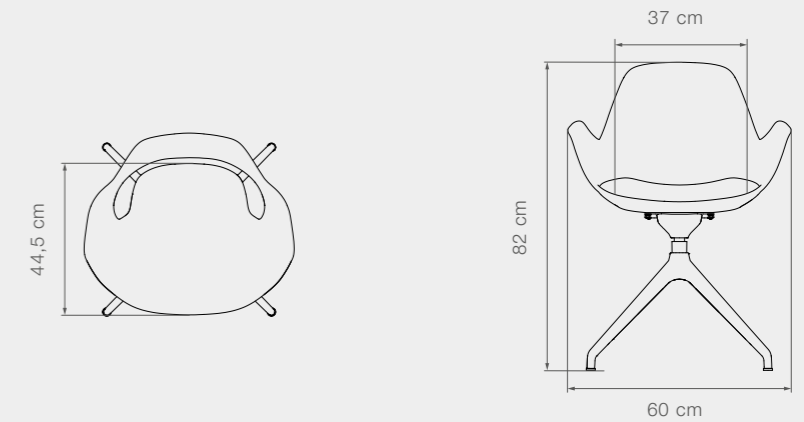
12901+12903 FALK Chair with four star return swivel base
