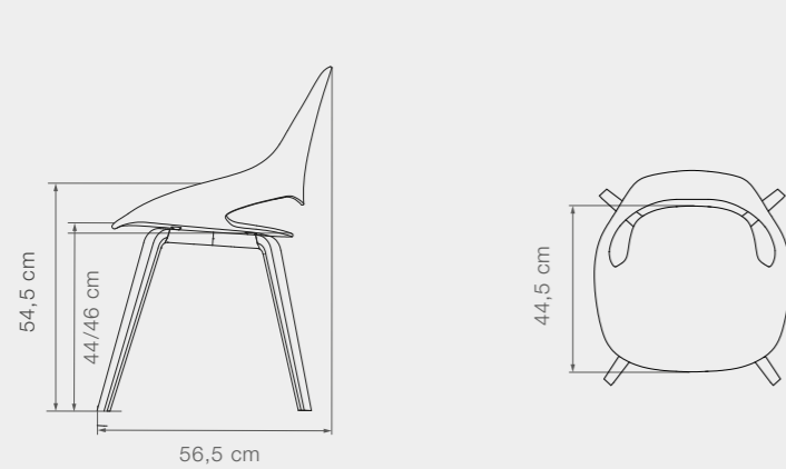
12902+12904 FALK Chair with oak veneer legs
