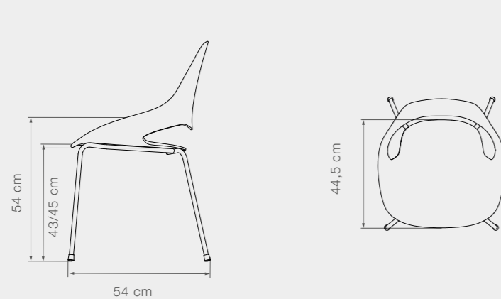
12902+12904 FALK Chair with tube legs
