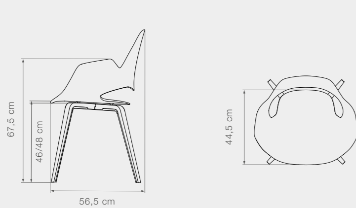
12901+12903 FALK Chair with oak veneer legs
