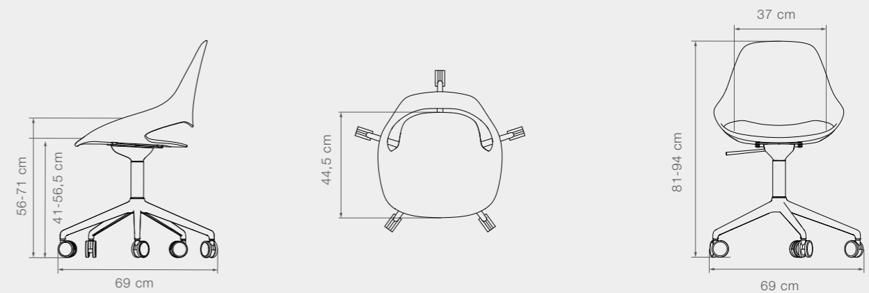
12902+12904 FALK Chair with five star castor base
